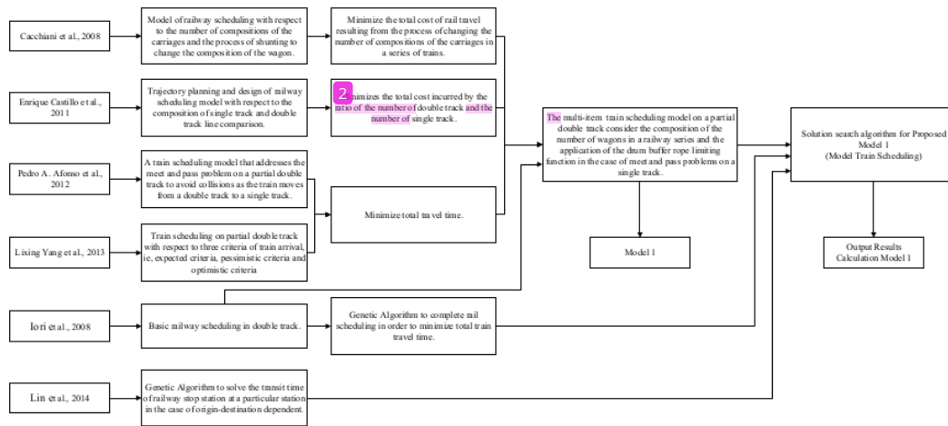
Fig. 2. Model Development of Railway Scheduling
