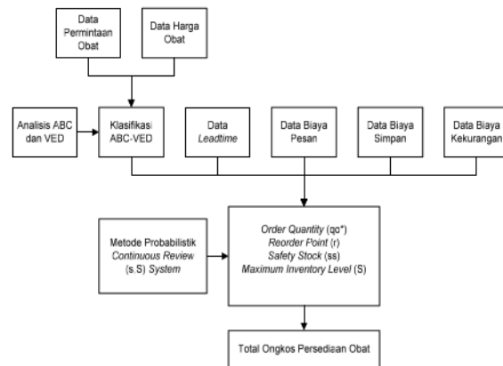
Gambar 1 Model konseptual
